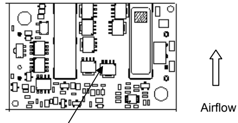
Figure 14. T_{ref} Temperature measurement location.
