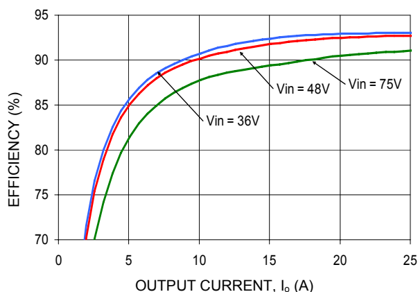
Figure 2. Converter Efficiency Vs Load at V_o = 3.3 V.
