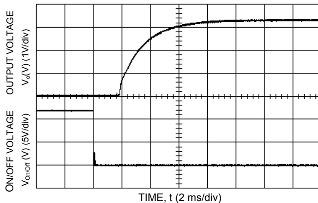
Figure 4. Typical Start-Up Characteristics from Remote ON/OFF.
