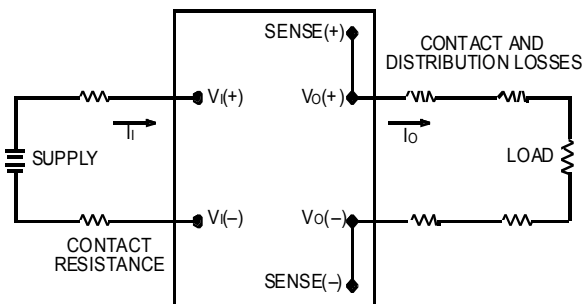
Figure 9. Output Voltage and Efficiency Test Setup.
