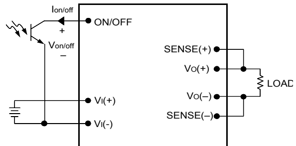
Figure 10. Circuit configuration for using Remote On/Off Implementation.
