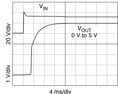
TURN ON RESPONSE MHV2805S
