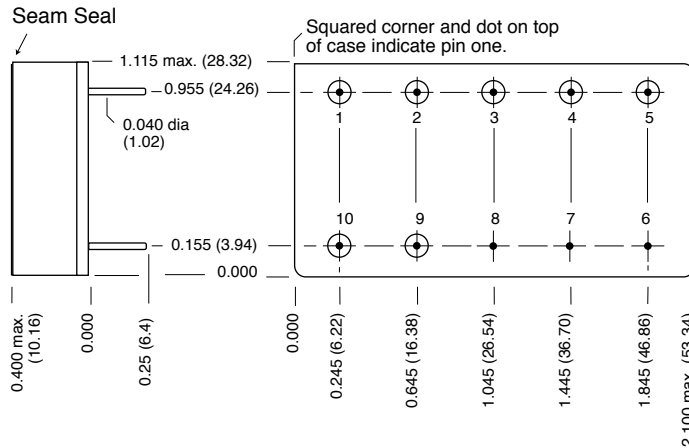
BOTTOM VIEW CASE H2
