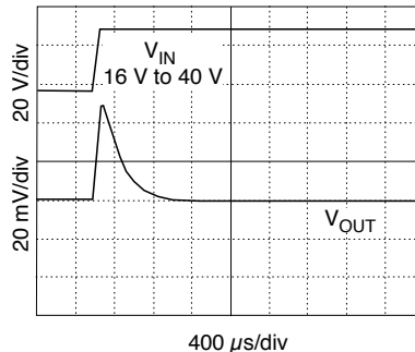
STEP LINE RESPONSE MHV2805S
