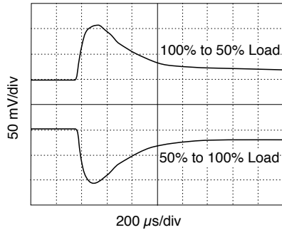
STEP LOAD RESPONSE MHV2805S
