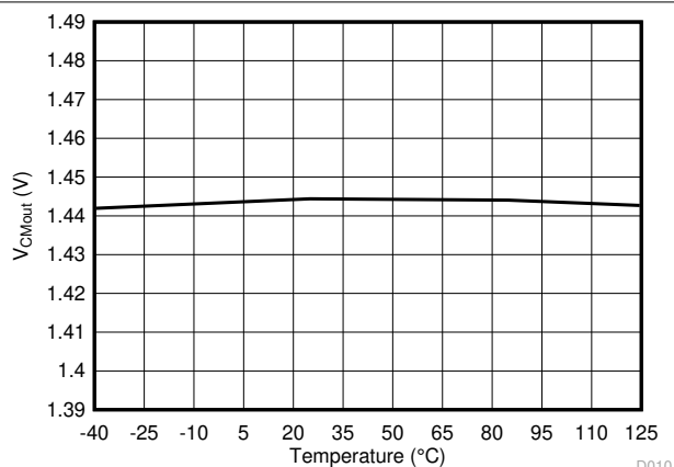
图 6-10. Output Common-Mode Voltage vs Temperature
