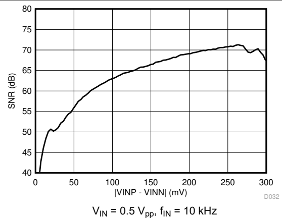
图 6-22. Signal-to-Noise Ratio vs Input Voltage
