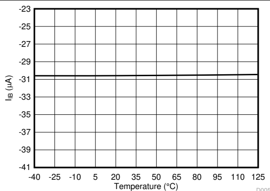
图 6-7. Input Bias Current vs Temperature
