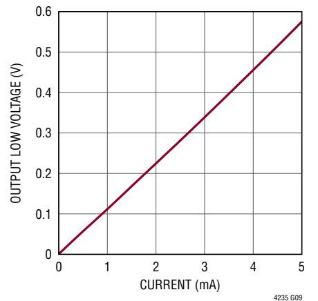
FAULT, PWRGD Output Low Voltage vs Current
