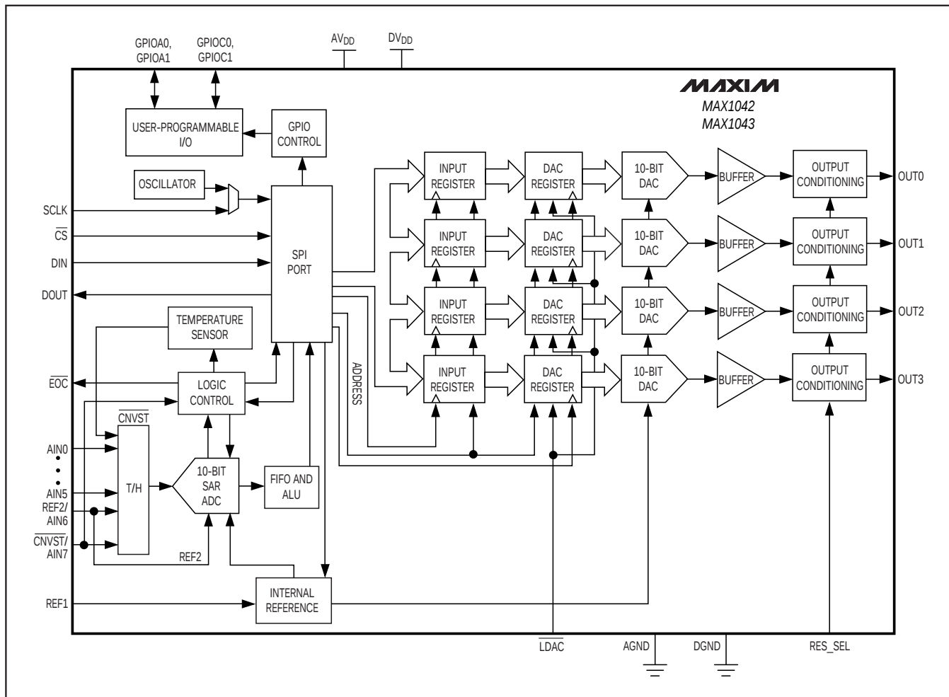
Figure 1. MAX1042/MAX1043 Functional Diagram
