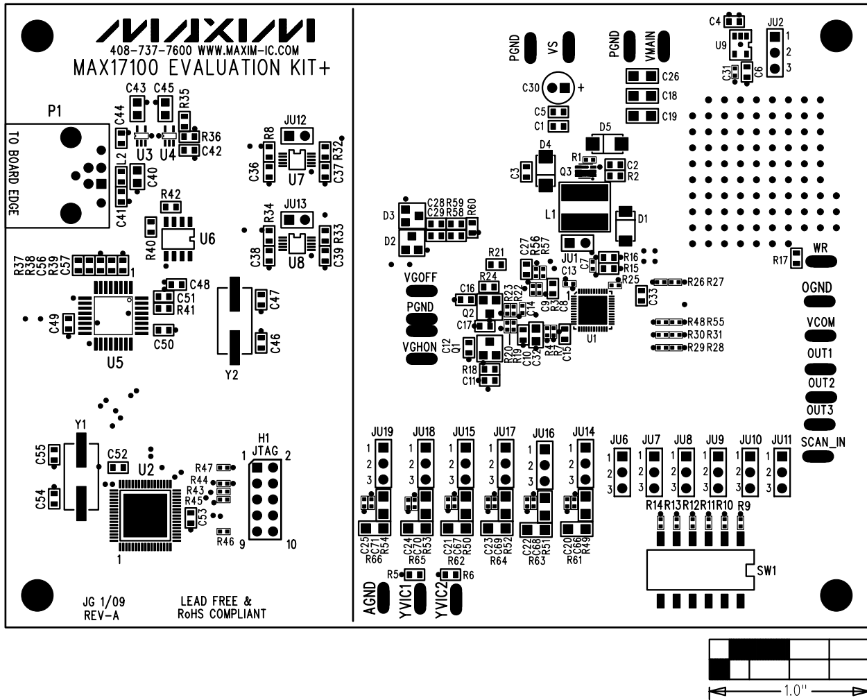
Figure 4. MAX17100 EV Kit Component Placement Guide—Component Side
