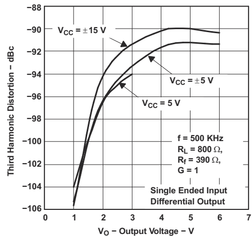
图 7-50. Third-Harmonic Distortion vs Output Voltage
