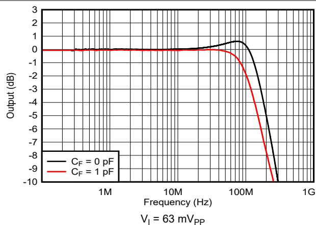
图 7-4. Small-Signal Frequency Response
