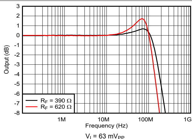
图 7-2. Small-Signal Frequency Response
