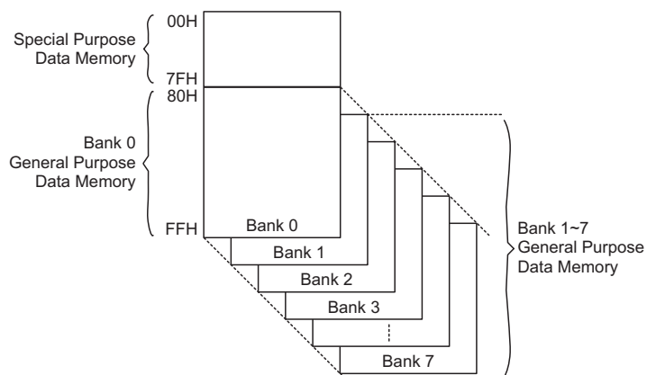
HT48R069B
