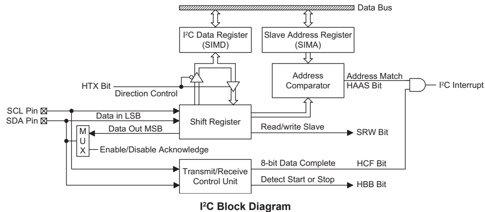
I²C Block Diagram
