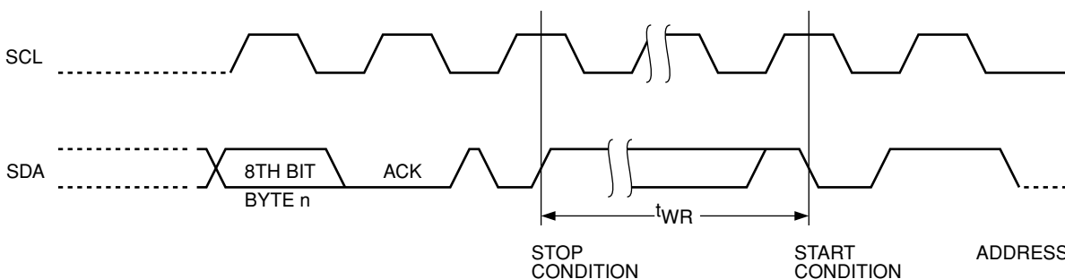
Figure 3. Start/Stop Timing
