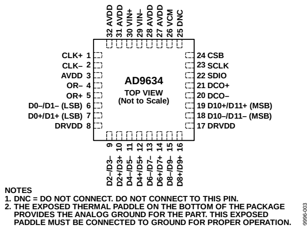
Figure 3. Pin Configuration
