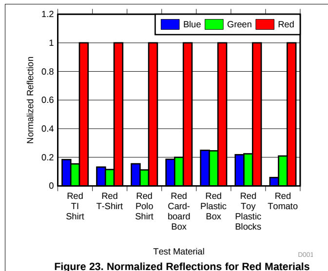
Figure 23. Normalized Reflections for Red Materials
