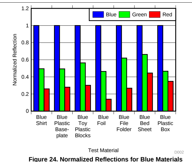
Figure 24. Normalized Reflections for Blue Materials
