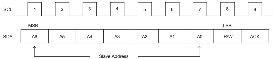
Figure 4: I²C Address Bit Map; 7-bit Slave Address (A6-A0), 1-bit Read/Write (R/W), 1-bit Acknowledge (ACK).
