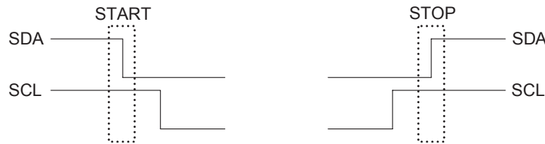
Figure 3: I²C Start and Stop Conditions.
