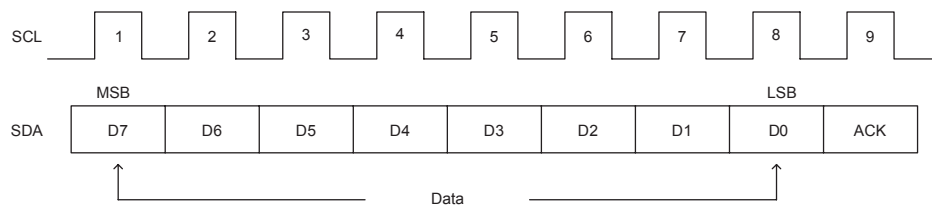
Figure 5: I²C Data Bit Map; 8-bit Data (D7-D0), 1-bit Acknowledge (ACK).
