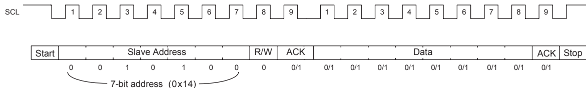
Figure 6: I²C SCL, SDA Transfer Protocol Example; 7-bit Slave Address (A6-A0 = 0x14), 1-bit Read/Write (R/W = 0), 1-bit Acknowledge (ACK), 8-bit Data (D7-D0), 1-bit Acknowledge (ACK).
