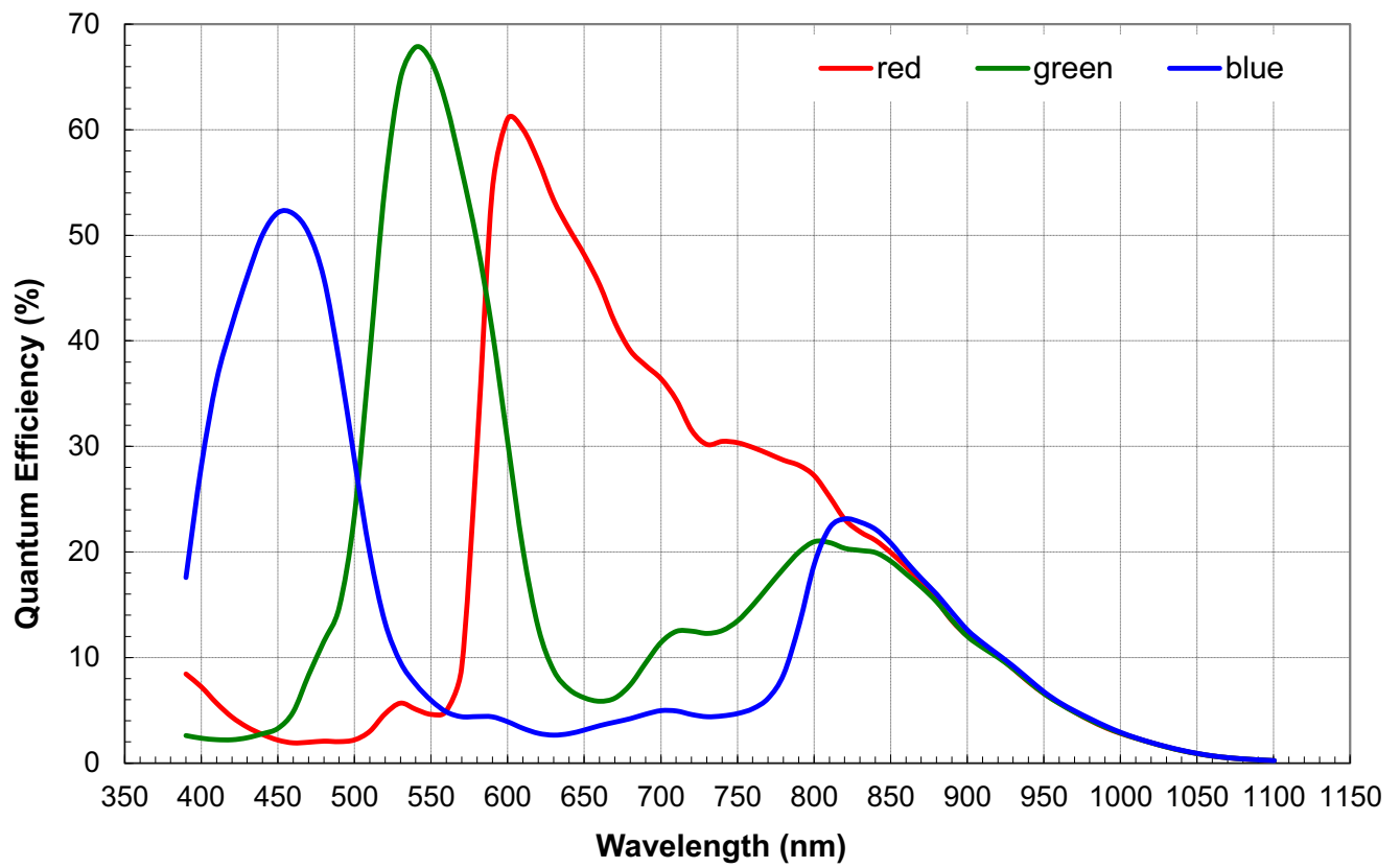
Figure 40: Quantum Efficiency - Color Sensor
