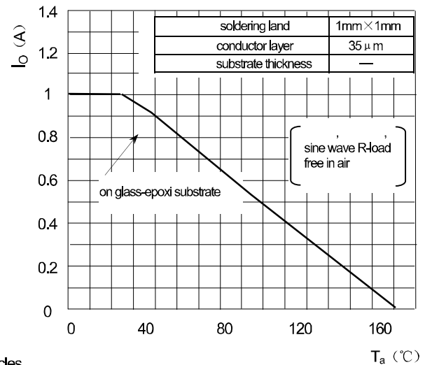
I_O-T_a Curve
