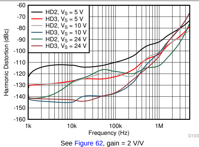
Figure 45. Harmonic Distortion vs Frequency vs Supply Voltage
