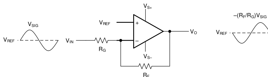
Figure 63. Inverting Amplifier
