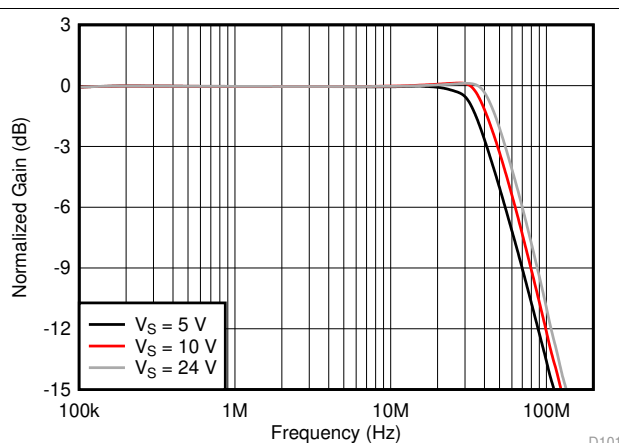
Figure 43. Large-Signal Response vs Supply Voltage
