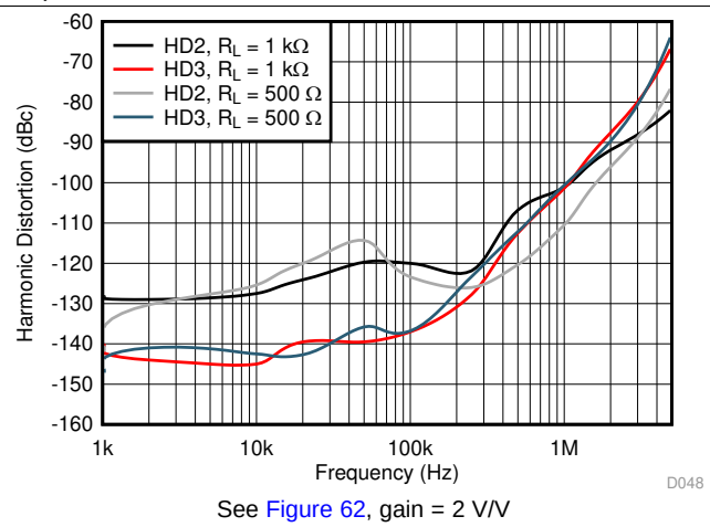
Figure 8. Harmonic Distortion vs Frequency
