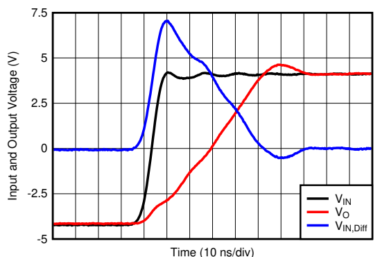
Figure 79. Large-Signal Transient Response Using the OPA810
