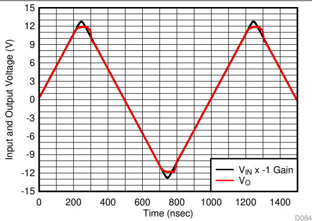
Figure 30. Output Overdrive Recovery
