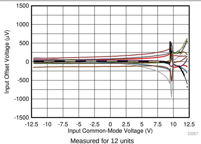
Figure 33. Input Offset Voltage vs Input Common-Mode Voltage
