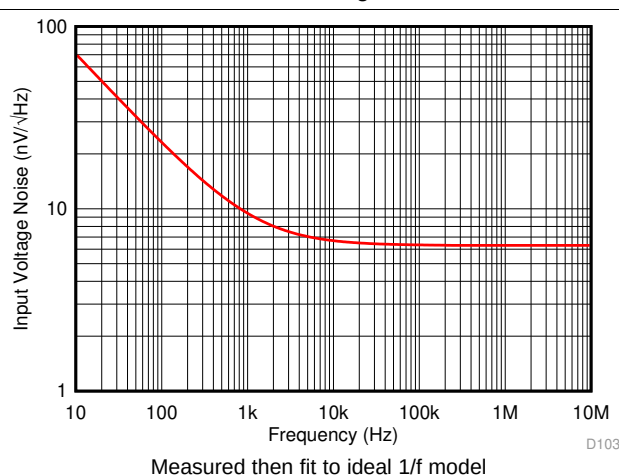
Figure 47. Input Voltage Noise Density vs Frequency
