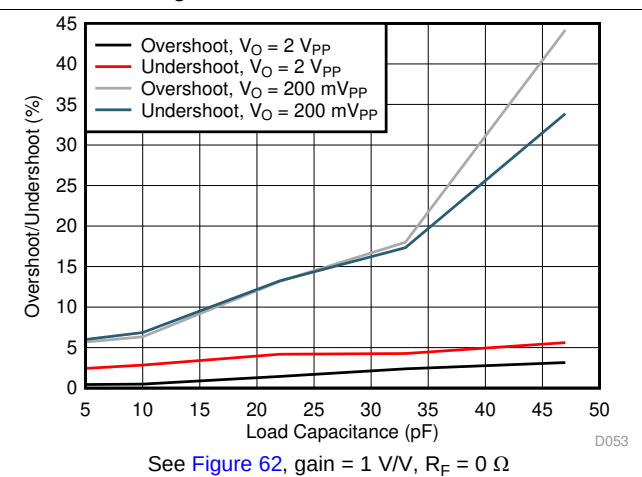
Figure 12. Overshoot and Undershoot vs C_L
