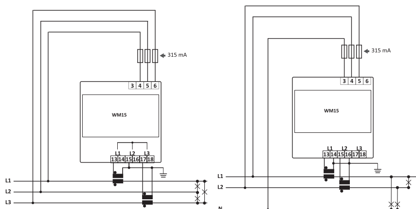
Fig. 7 Three-phase without neutral (3-wire)
