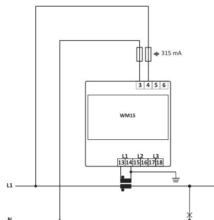
Fig. 9 Single-phase (2-wire)
