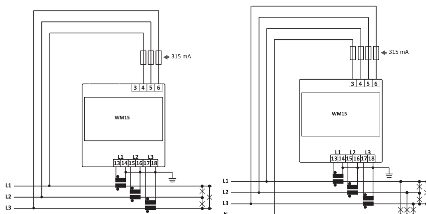
Fig. 5 Three-phase without neutral (3-wire)
