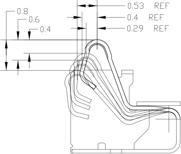
SECTION B-B STROKE CONDITION(REFERENCE)
