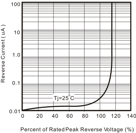
Fig. 1 - Reverse Characteristics
