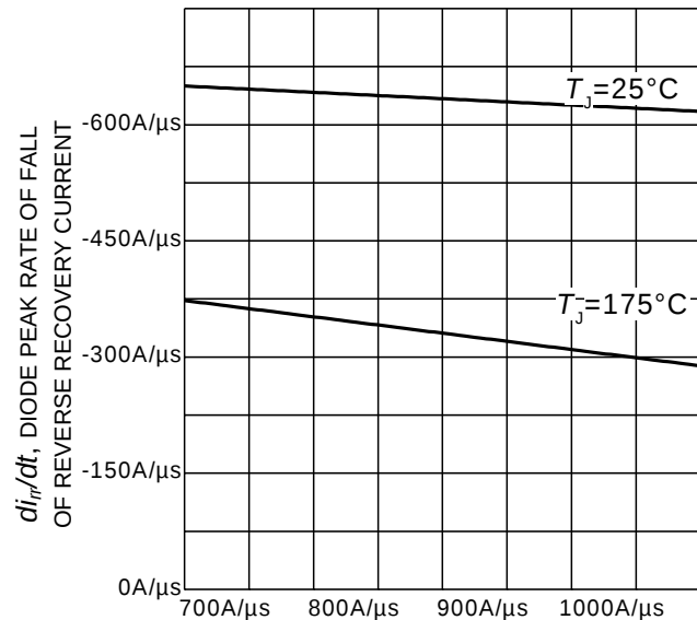
Figure 26. Typical diode peak rate of fall of reverse recovery current as a function of diode current slope ( V_R = 400\text{V} , I_F = 30\text{A} , Dynamic test circuit in Figure E)
