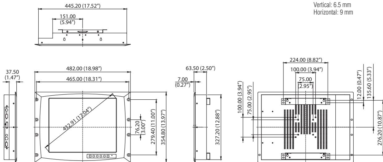
Panel Cut-out Dimensions: FPM-3171G: 447.5 x 329.5 mm (17.62" x 12.97")
