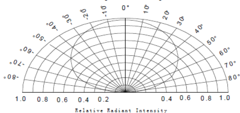
Fig.7 Radiation diagram
