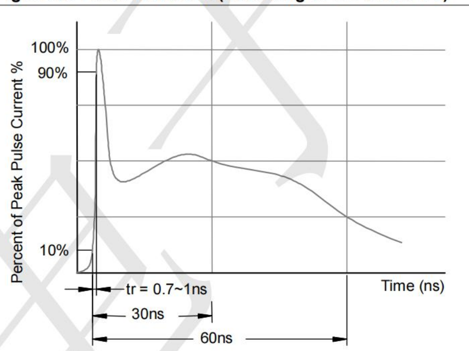
Fig2. ESD Pulse Waveform (according to IEC 61000-4-2)
