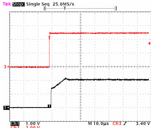
FIGURE 57. TURN-ON TIME, 1k \Omega
