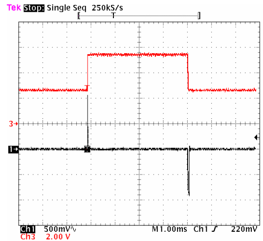
FIGURE 60. LINE TRANSIENT RESPONSE, 1nF LOAD
