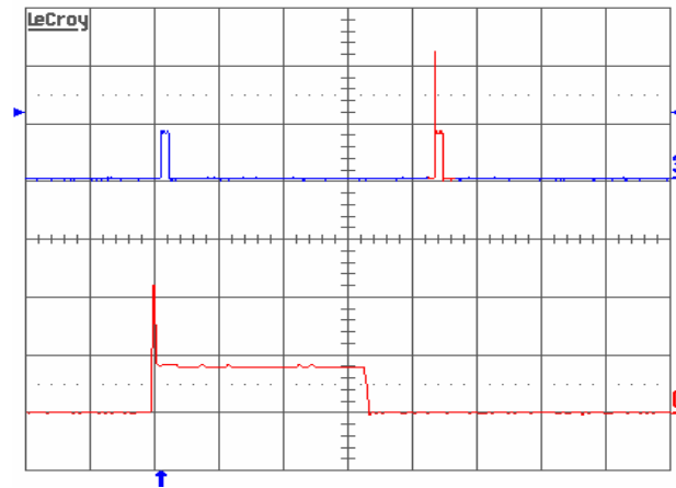
Figure 14. Load current (top trace, 5A/div., 50ms/div.) into a 10m short circuit during restart, at V_{in} = 48V . Bottom trace (5A/div., 2ms/div.) is an expansion of the on-time portion of the top trace
