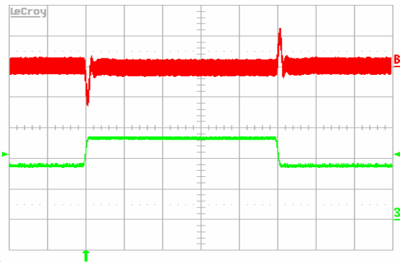
Figure 8. Output voltage response to load current step- (3.5A–5.25A–3.5A) at V_{in} =48V. Top trace: output voltage (100mV/div.) Bottom trace: load current (2A/div.). Current slew rate: 0.1A/ \mu s. C_o =1 \mu F ceramic + 10 \mu F tantalum. Time scale: 0.2ms/div.
