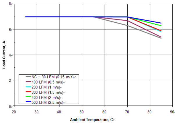
Figure 1. Available load current vs. ambient air temperature and airflow rates for SSQE48S07120 converter mounted vertically with air flowing from pin 1 to pin 3, V_{in} = 48V . Note: NC – Natural convection
