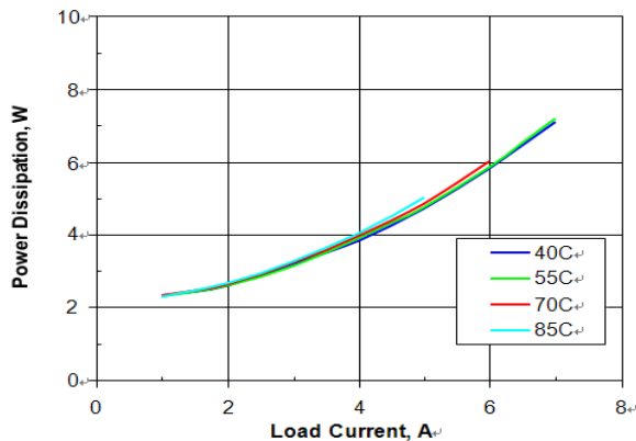
Figure 5. Power dissipation vs. load current and ambient temperature for SSQE48S07120 converter mounted vertically with V_{in} = 48V and air flowing from pin 1 to pin 3 at a rate of 200 LFM (1.0 m/s).
