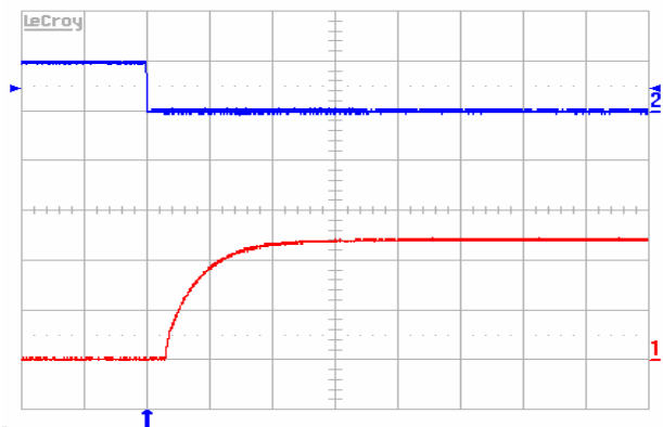
Figure 6. Turn-on transient at full rated load current (resistive) with no output capacitor at V_{in} = 48V , triggered via ON/OFF pin. Top trace: ON/OFF signal (5V/div.). Bottom trace: Output voltage (5V/div.). Time scale: 2ms/div.
