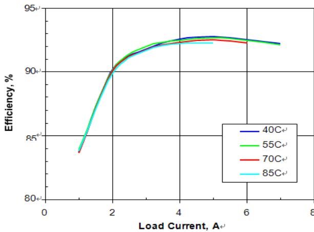
Figure 3. Efficiency vs. load current and ambient temperature for SSQE48S07120 converter mounted vertically with V_{in} = 48V and air flowing from pin 1 to pin 3 at a rate of 200 LFM (1.0 m/s).
