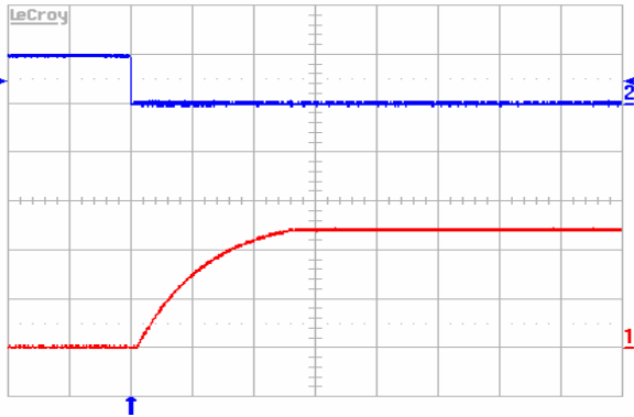
Figure 7. Turn-on transient at full rated load current (resistive) plus 3,300 \mu F at V_{in} = 48V, triggered via ON/OFF pin. Top trace: ON/OFF signal (5V/div.). Bottom trace: Output voltage (5V/div.). Time scale: 2ms/div.
