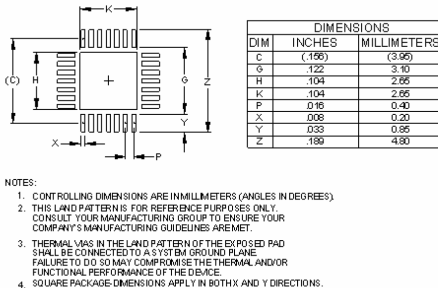
Figure 63 Land Pattern
