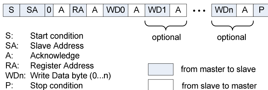
Figure 55 I2C write
