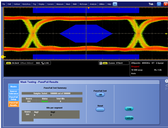
Mask testing an OC-12 signal, capturing any violations of the mask.
