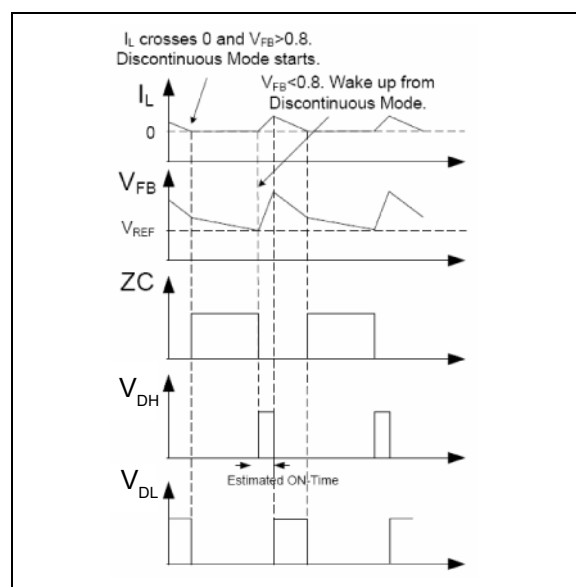
FIGURE 4-3: MIC2103 Control Loop Timing (Discontinuous Mode).
