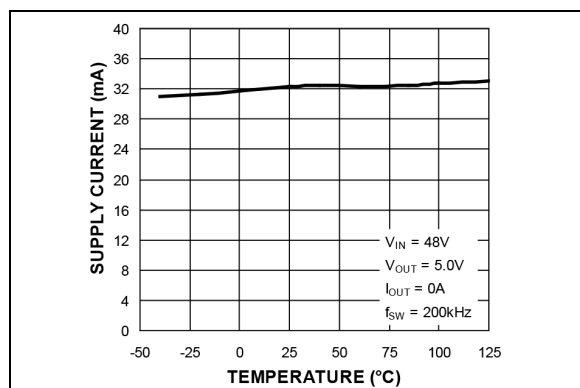
FIGURE 2-20: V_{IN} Operating Supply Current vs. Temperature (MIC2104).
