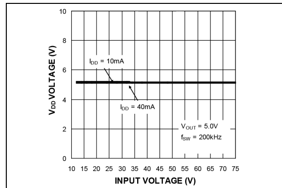
FIGURE 2-35: V_{DD} Voltage vs. Input Voltage.
