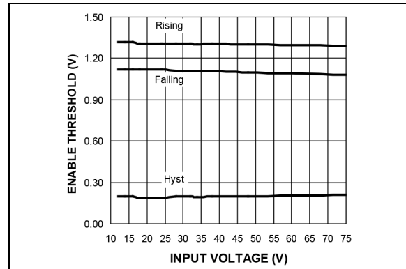
FIGURE 2-36: Enable Threshold vs. Input Voltage.
