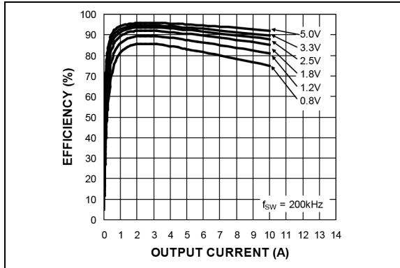
FIGURE 2-25: Efficiency ( V_{IN} = 12\text{V} ) vs. Output Current (MIC2104).
