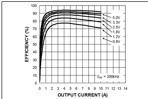
FIGURE 2-27: Efficiency ( V_{IN} = 24\text{V} ) vs. Output Current (MIC2104).
