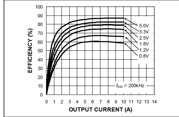
FIGURE 2-30: Efficiency ( V_{IN} = 75\text{V} ) vs. Output Current (MIC2104).
