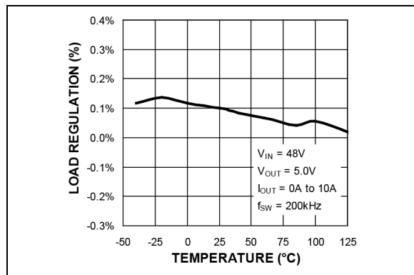
FIGURE 2-21: Load Regulation vs. Temperature (MIC2104).
