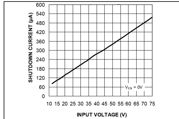
FIGURE 2-34: V_{IN} Shutdown Current vs. Input Voltage.
