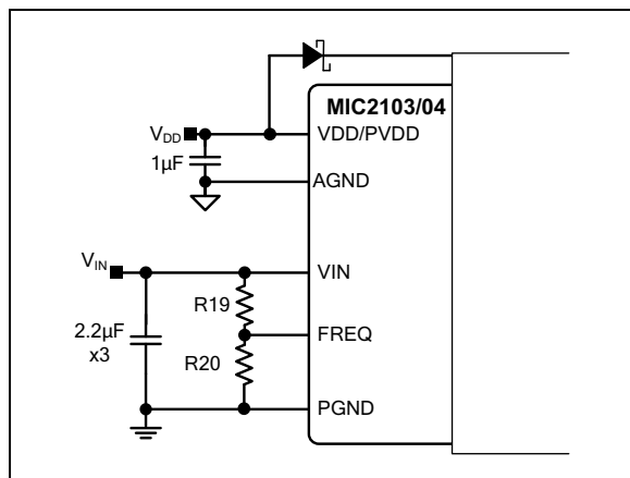
FIGURE 5-1: Switching Frequency Adjustment.
