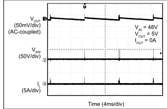
FIGURE 2-66: MIC2103 Switching Waveforms ( I_{OUT} = 0A , DCM).
