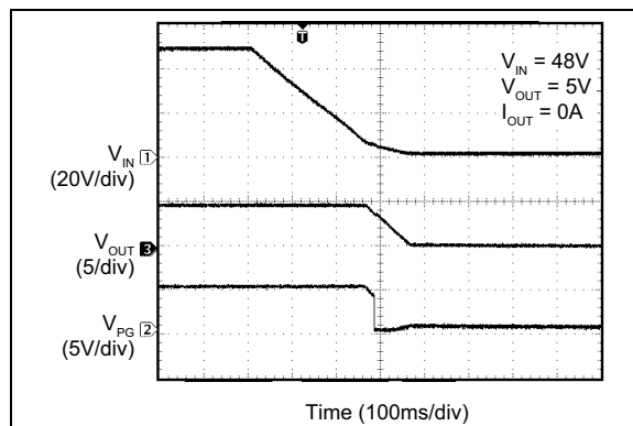
FIGURE 2-74: Power Good at V_{IN} Soft Turn-Off.
