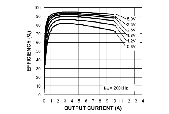
FIGURE 2-26: Efficiency ( V_{IN} = 18\text{V} ) vs. Output Current (MIC2104).
