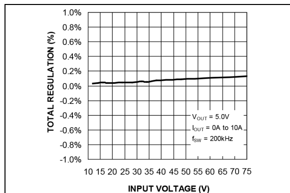
FIGURE 2-19: Output Regulation vs. Input Voltage (MIC2104).
