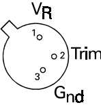
Bottom View – Case is internally connected to pin 3
