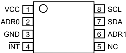
Package LE, 8-Pin TSSOP Pinout Diagram
