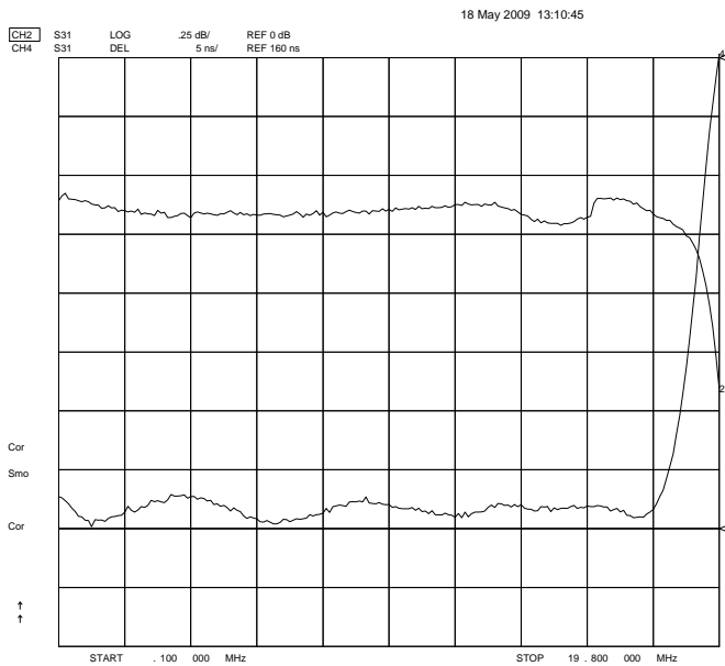
Passband Response (0.25 dB/div & 5 nsec/div)
