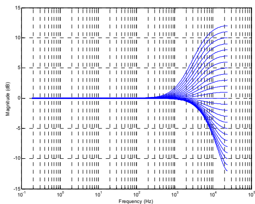
Figure 67 EQ Band 5 Gains for Lowest Cut-off Frequency
