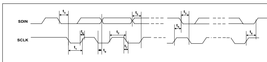
Figure 7 Control Interface Timing – 2-Wire Serial Control Mode
