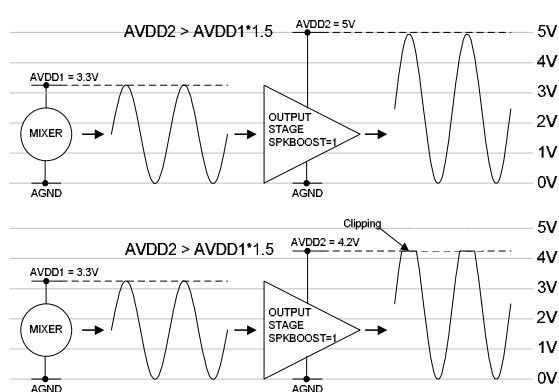
Figure 27 Boost Mode Output Operation
