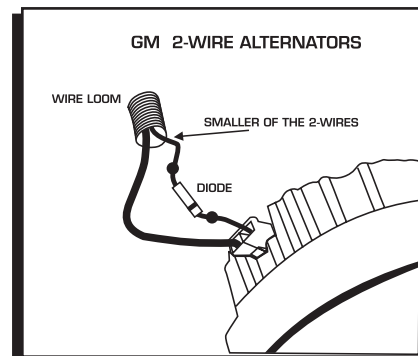
Figure 10 Installing the Diode to a 1973-1983 GM Vehicle.
