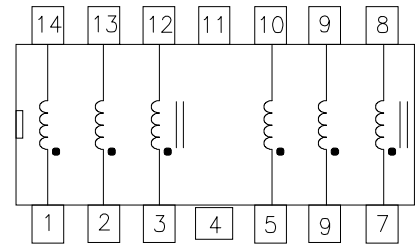
Schematic Diagram
