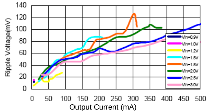
ACE701140AM+ Ripple Voltage VS. Output Current
