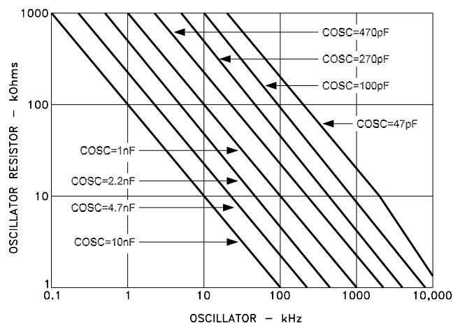
OSCILLATOR FREQUENCY COMPONENT SELECTION FOR MSK4351-1
