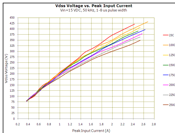
Chart 4. Vdss vs. Peak Input Current
