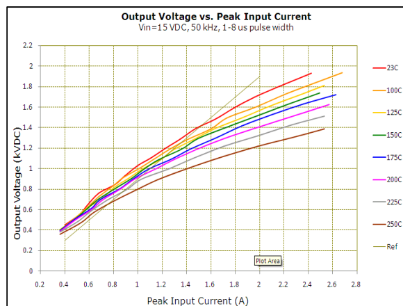
Chart 2. Output Voltage vs. Peak Input Current
