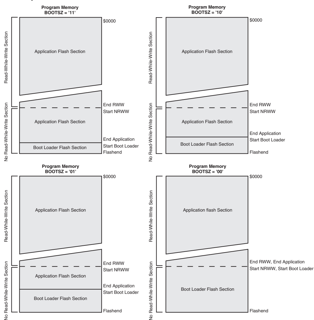
Figure 24-2. Memory Sections (1)
