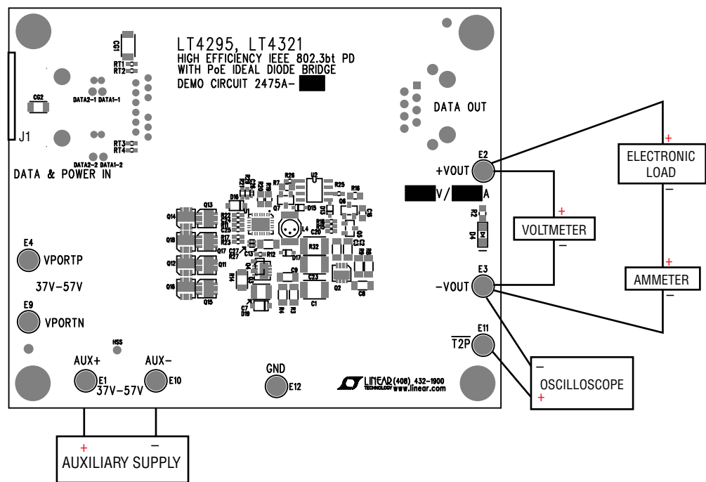
Figure 9: Setup Diagram for Auxiliary Supply Input
