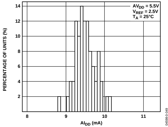
Figure 15. I_{DD} Histogram
