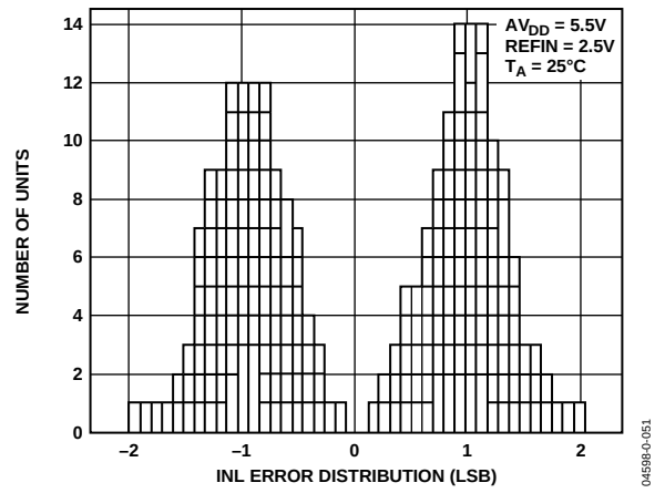
Figure 19. INL Error Distribution
