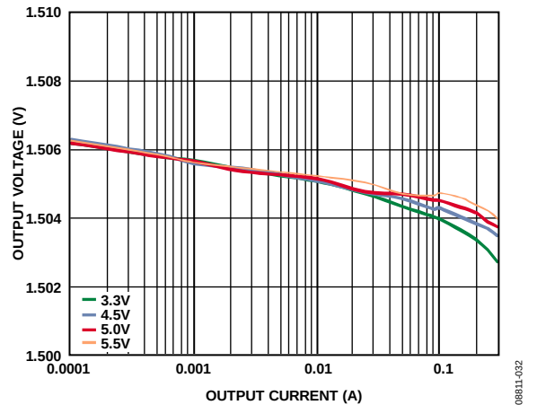
Figure 32. LDO1 Load Regulation Across Input Voltage, VOUT2 = 1.5 V
