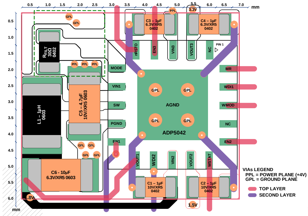
Figure 68. Layout
