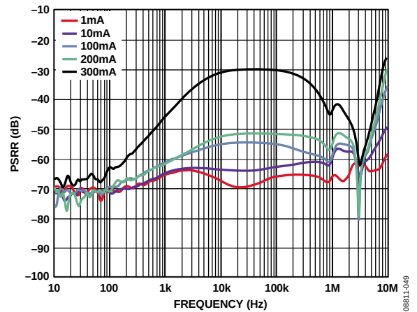
Figure 50. LDO2 PSRR Across Output Load, VIN3 = 3.3 V, VOUT3 = 2.8 V
