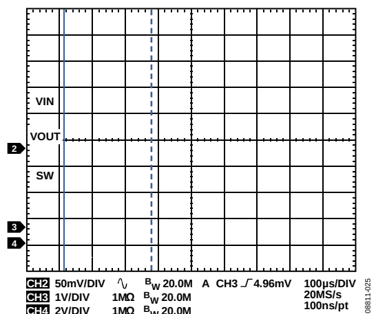
Figure 25. Buck Response to Line Transient, V IN = 4.5 V to 5.0 V, VOUT1 = 1.8 V, PWM Mode
