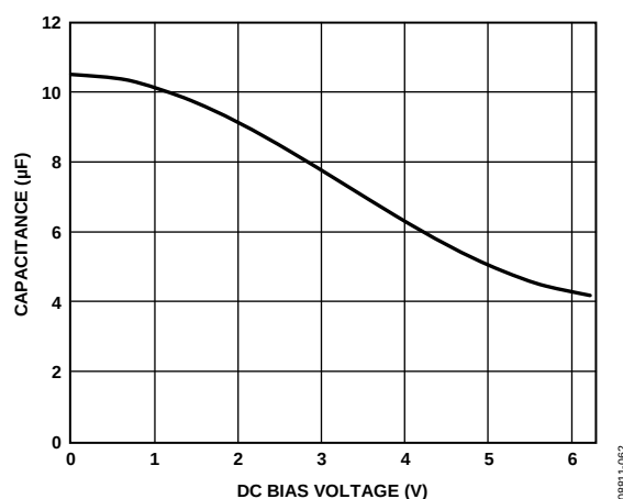
Figure 61. Typical Capacitor Performance
