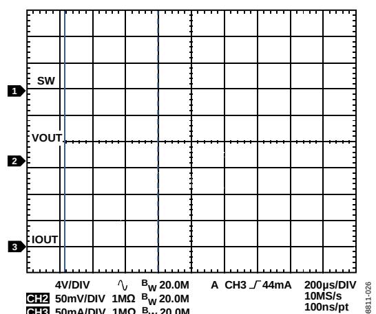
Figure 26. Buck Response to Load Transient, IOUT1 from 1 mA to 50 mA, VOUT1 = 3.3 V, Auto Mode
