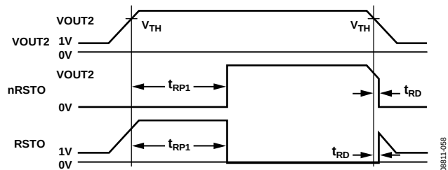
Figure 57. Reset Timing Diagram
