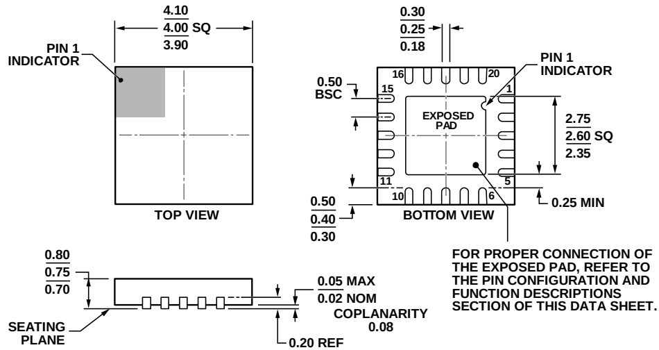
Figure 70. 20-Lead Lead Frame Chip Scale Package [LFCSP_WQ] 4 mm × 4 mm Body, Very Very Thin Quad (CP-20-8) Dimensions shown in millimeters
