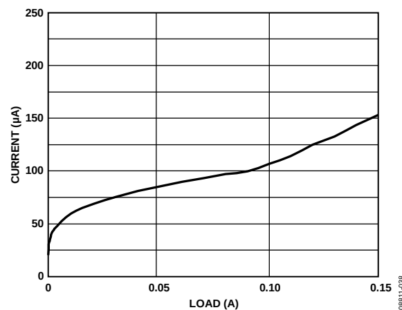
Figure 38. LDO2 Ground Current vs. Output Load, VOUT3 = 2.8 V
