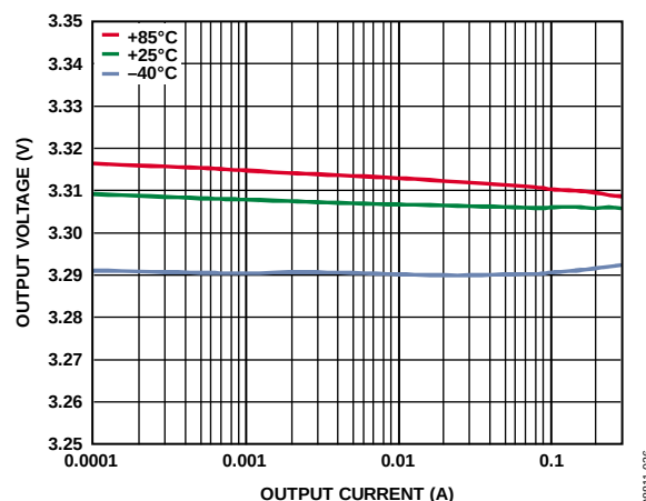
Figure 36. LDO2 Load Regulation Across Temperature, VIN3 = 3.6 V, VOUT3 = 3.3 V
