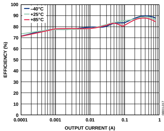
Figure 17. Buck Efficiency vs. Load Current, Across Temperature, V_{OUT1} = 1.8\text{ V} , Auto Mode
