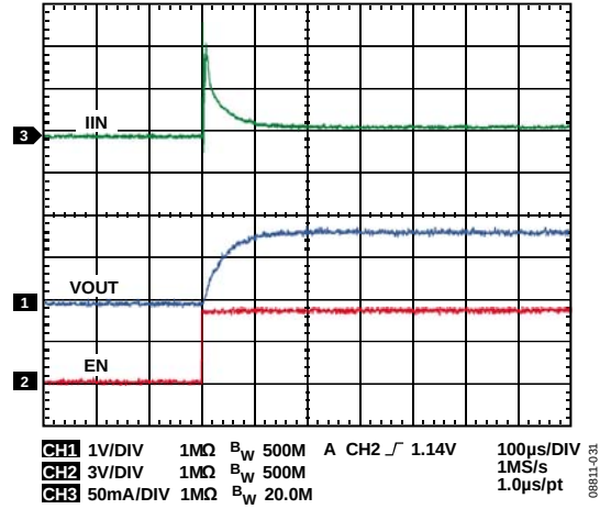
Figure 31. LDO2 Startup, VOUT3=3.3 V, IOUT3 = 5 mA
