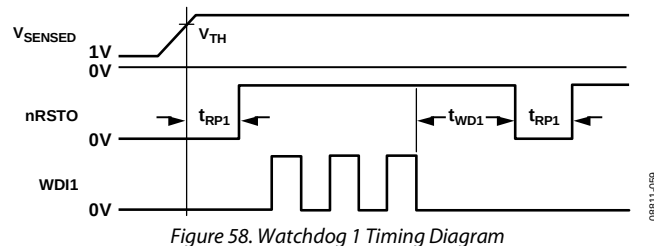
Figure 58. Watchdog 1 Timing Diagram
