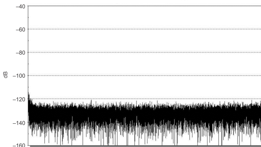
Figure 43. FFT plot- Noise floor of Data Acquisition system
