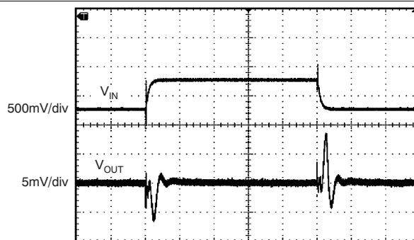
20µs/div ( C_L = 1\text{ }\mu\text{F} )
