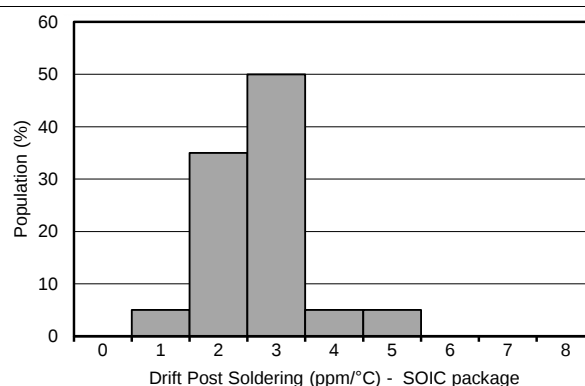
Figure 32. Drift Post Soldering Distribution, SOIC Package
