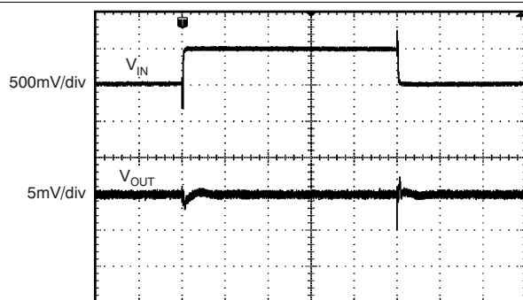
100µs/div ( C_L = 10\text{ }\mu\text{F} )
