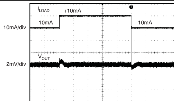
100µs/div ( C_L = 10\text{ }\mu\text{F} , I_{\text{OUT}} = 10\text{ mA} )
