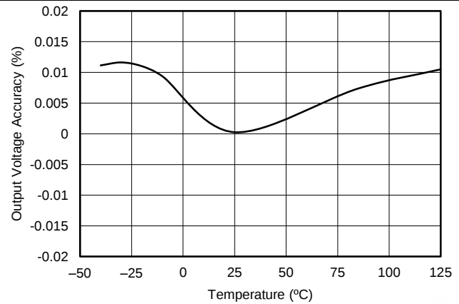
Figure 2. Temperature Drift
