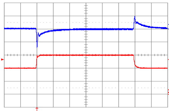
Fig. 9: Output voltage response to load current step-change (20 A – 30 A – 20 A) at V_{in} = 48\text{ V} . Top trace: output voltage (100 mV/div.). Bottom trace: load current (10 A/div.). Current slew rate: 1 A/ \mu\text{s} . C_o = 470\text{ }\mu\text{F} tantalum + 1 \mu\text{F} ceramic. Time scale: 0.2 ms/div.
