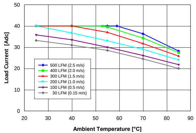
Fig. 2: Available load current vs. ambient air temperature and airflow rates for QM48T40033 converter with B height pins mounted horizontally with air flowing from pin 3 to pin 1, MOSFET temperature \leq 120^{\circ}\text{C} , V_{in} = 48\text{ V} .
