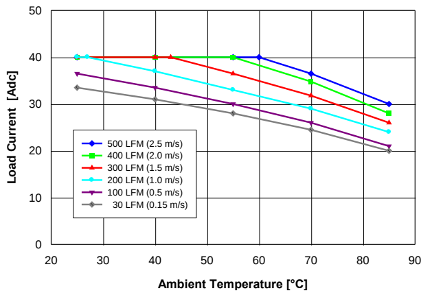
Fig. 1: Available load current vs. ambient air temperature and airflow rates for QM48T40033 converter with B height pins mounted vertically with air flowing from pin 3 to pin 1, MOSFET temperature \leq 120^{\circ}\text{C} , V_{in} = 48\text{ V} .
