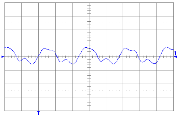
Fig. 10: Output voltage ripple (20 mV/div.) at full rated load current into a resistive load with C_o = 10\text{ }\mu\text{F} tantalum + 1 \mu\text{F} ceramic and V_{in} = 48\text{ V} . Time scale: 1 \mu\text{s} /div.
