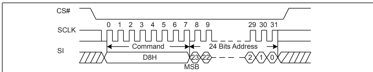
Figure 12. 64KB Block Erase Sequence Diagram
