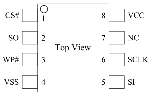
8-LEAD SOP
