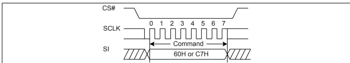
Figure 13. Chip Erase Sequence Diagram
