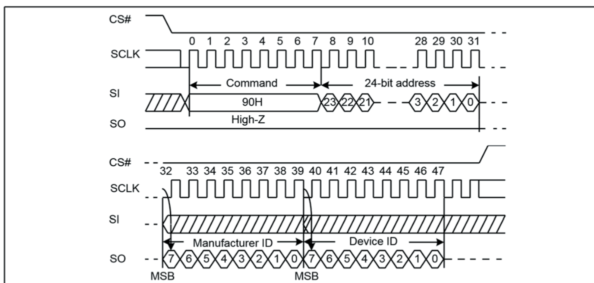
Figure 17. Read Manufacture ID/Device ID Sequence Diagram
