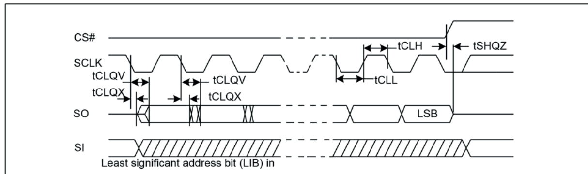
Figure 21. Output Timing
