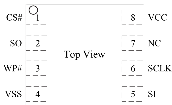
8-LEAD USON
