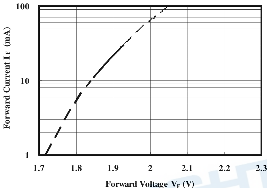
Forward Current vs. Forward Voltage (Ta=25°C)
