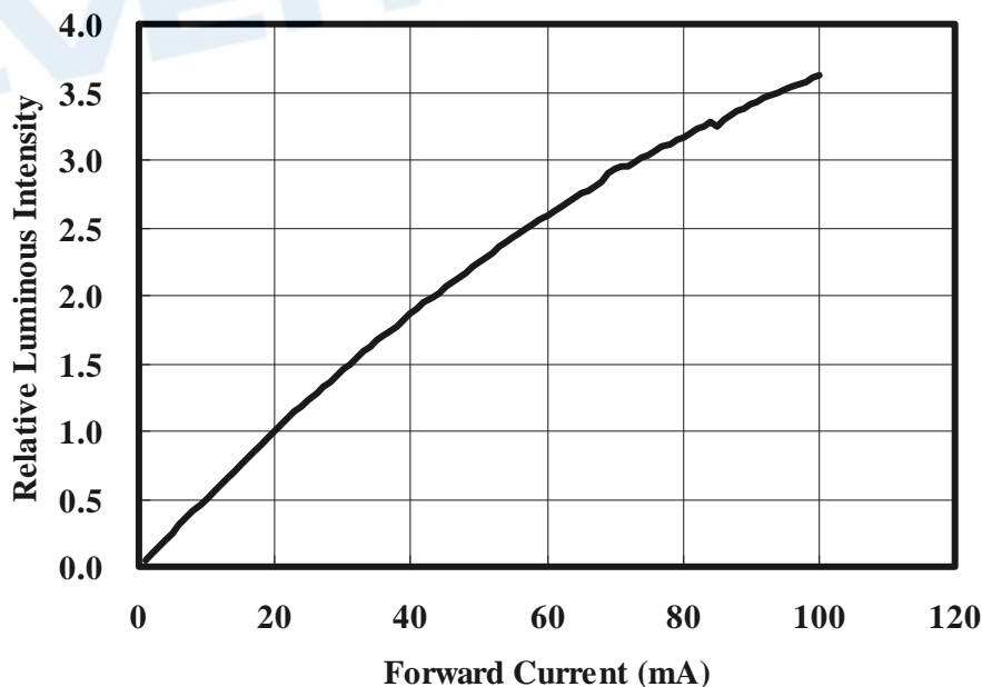
Relative Luminous Intensity vs. Forward Current (Ta=25°C)
