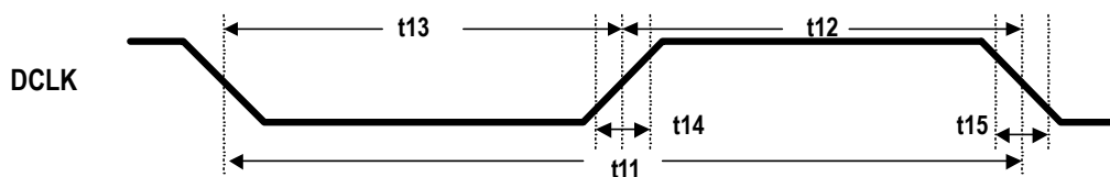
Figure 17. DCLK Timing in Mode '1'
