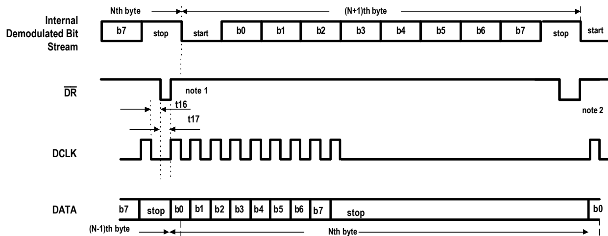
Figure 18. Serial Data Interface Timing in MODE '1'
