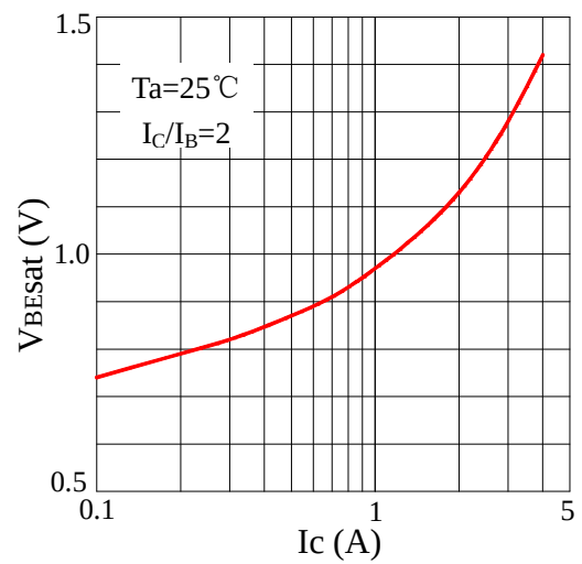
Fig4 V_{BEsat}-I_C
