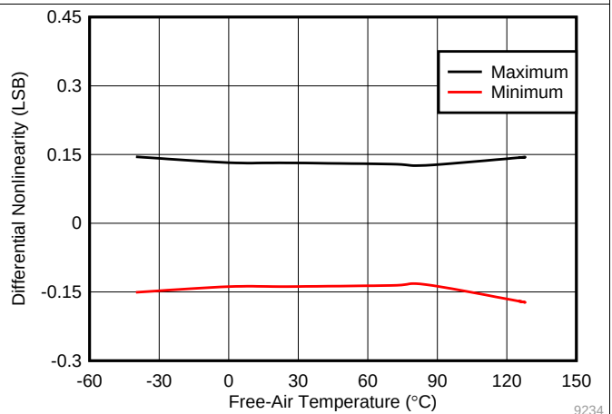
图 32. Typical DNL
