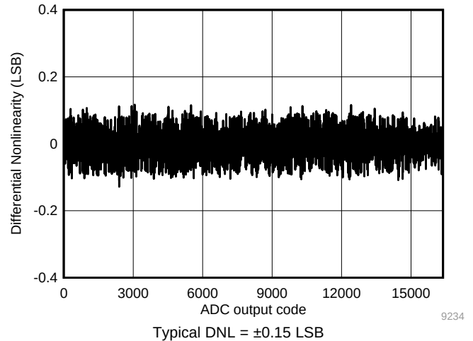
图 32. Typical DNL
