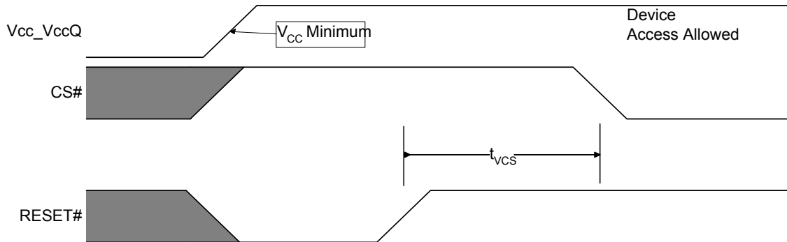
Figure 7.4 Power-up with RESET# Low
