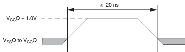
Figure 7.2 Maximum Positive Overshoot Waveform
