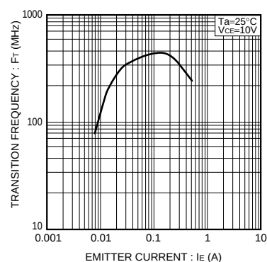
Fig.9 Transition frequency
