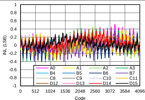
Figure 7. DAC Linearity Error vs Code DAC Range: 0 to 5 V
