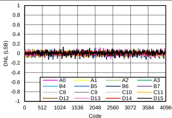
Figure 8. DAC Differential Linearity Error vs Code DAC Range: 0 to 5 V
