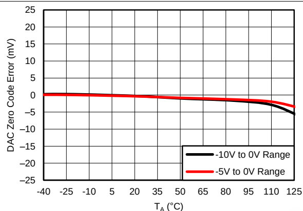
Figure 20. DAC Zero Code Error vs Temperature
