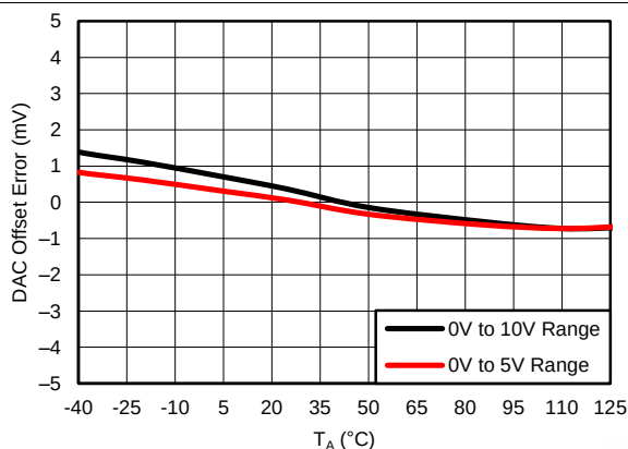
Figure 19. DAC Offset Error vs Temperature
