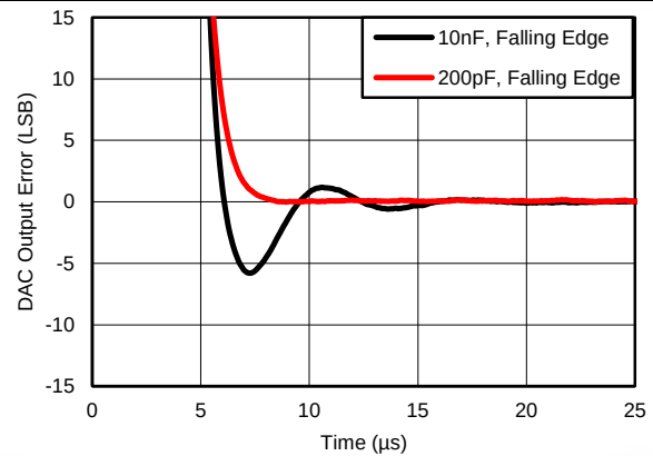
Figure 26. DAC Settling Time vs Load Capacitance
