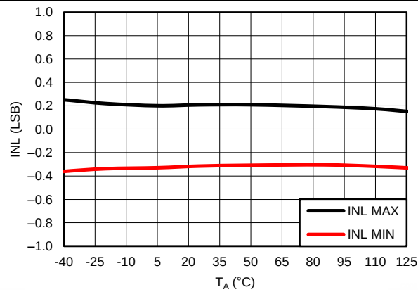
Figure 13. DAC Linearity Error vs Temperature DAC Range: -10 to 0 V
