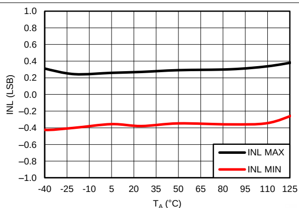
Figure 40. ADC Linearity Error vs Temperature Unipolar Input
