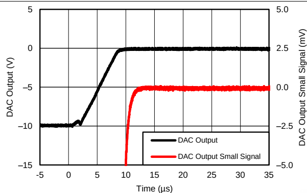
Figure 31. DAC Clamp Recovery
