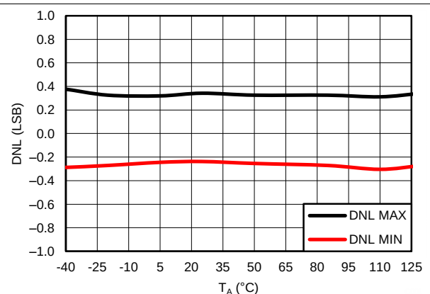
Figure 41. ADC Differential Linearity Error vs Temperature Unipolar Input
