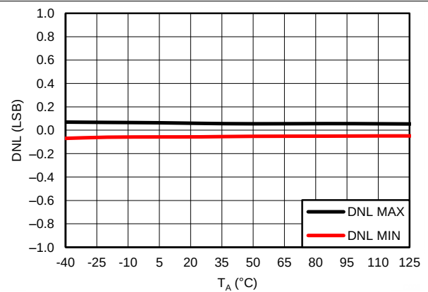
Figure 14. DAC Differential Linearity Error vs Temperature DAC Range: -10 to 0 V
