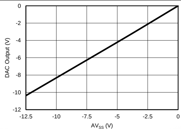
Figure 30. DAC Clamp Output vs AV_{SS}
