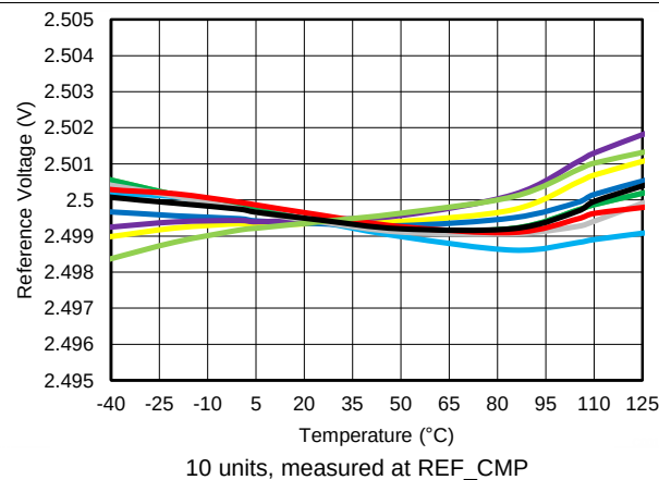
Figure 46. Reference Voltage vs Temperature
