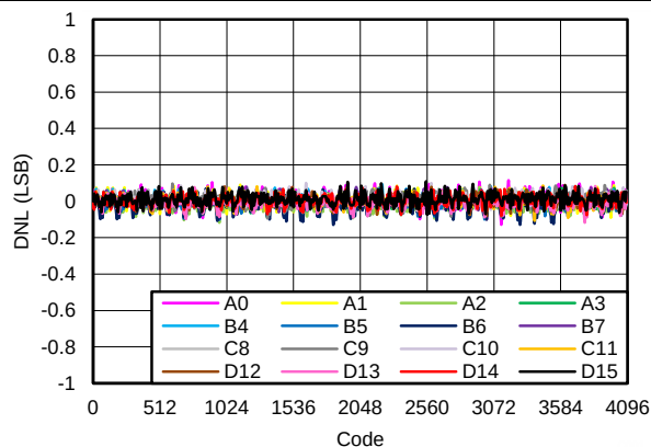
Figure 8. DAC Differential Linearity Error vs Code DAC Range: 0 to 5 V
