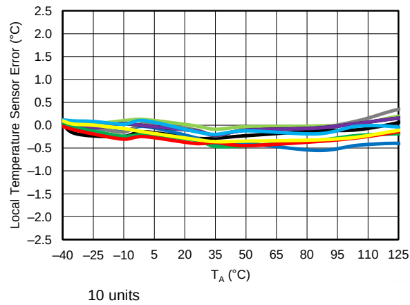
Figure 47. Temperature Sensor Error vs Temperature
