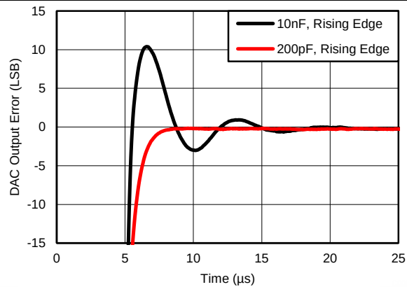
Figure 25. DAC Settling Time vs Load Capacitance
