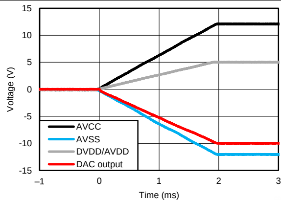
Figure 29. DAC Power On Overshoot, Dual Supply
